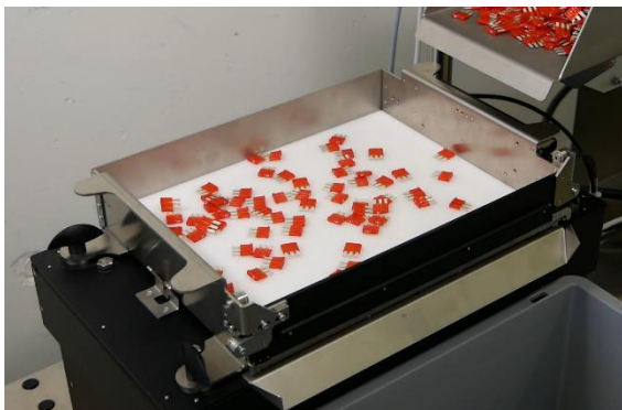
Asycube 380 with closed purge platform
